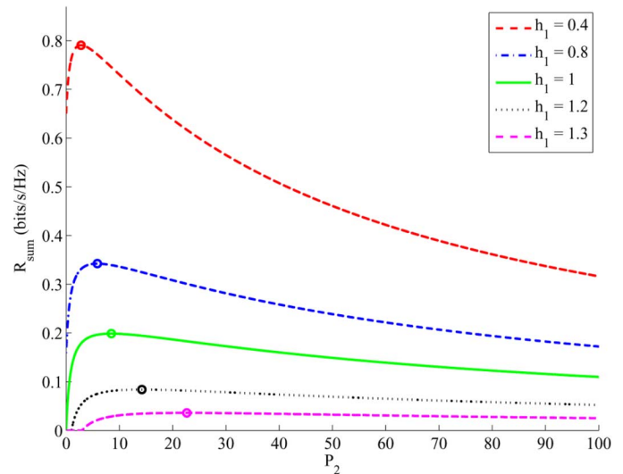
Fig. 8. GGMAC-WT cooperative jamming secrecy sum rate as a function of P_2 with different h_1 for \bar{P}_1 = \bar{P}_2 = 100 and h_2 = 1.4 . The circles indicate optimum jamming power.
