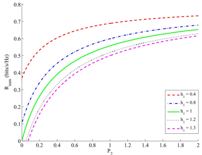
Fig. 9. GTW-WT cooperative jamming secrecy sum rate as a function of P_2 with different h_1 for \bar{P}_1 = \bar{P}_2 = 2 and h_2 = 4.2 .
